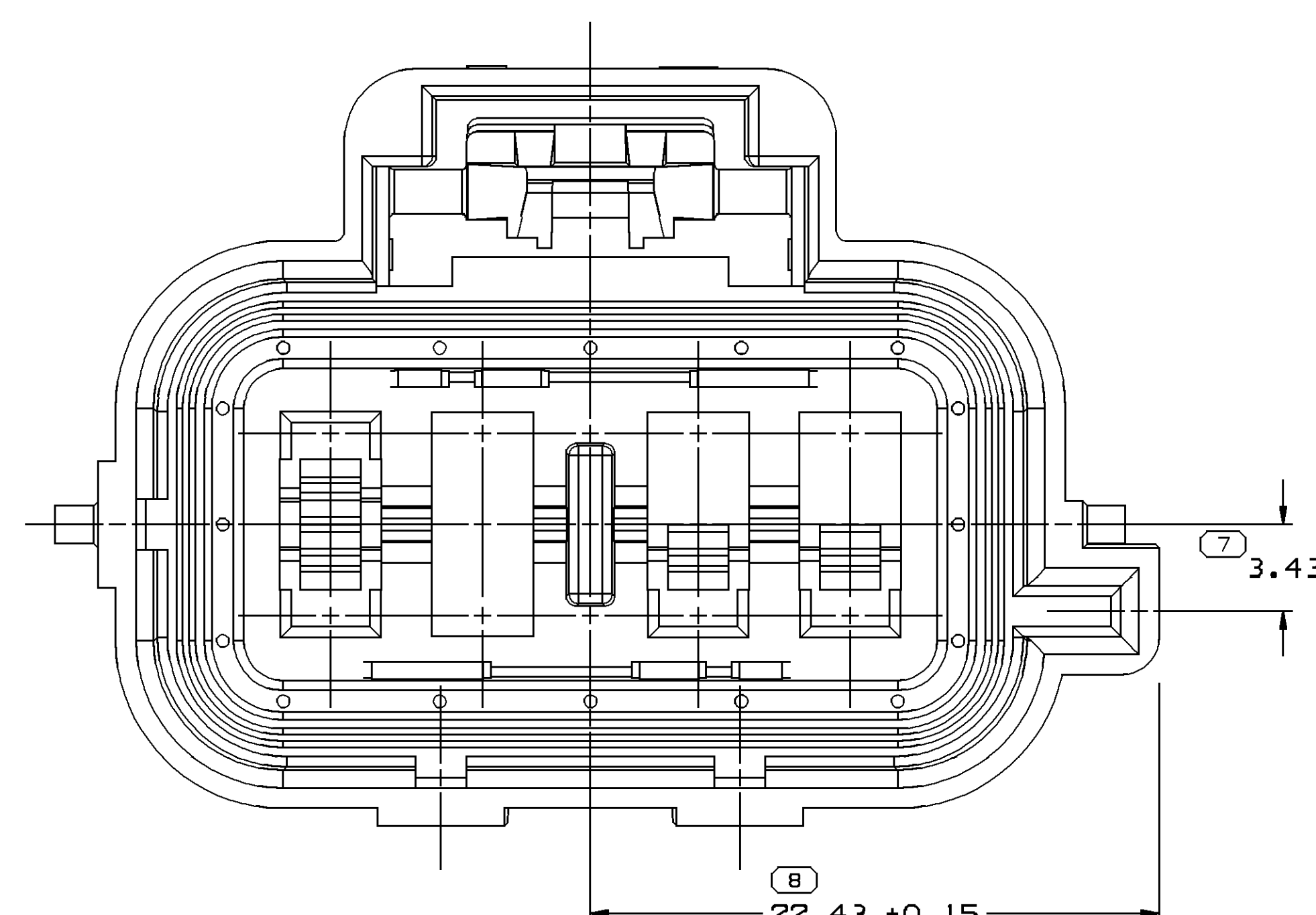
TYPE 104 SAME AS TYPE 103 EXCEPT AS SHOWN
